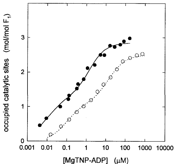
Fig. 3. Binding of MgTNP-ADP to catalytic sites of E. coli F_1 . Nucleotide binding was measured as described in Materials and Methods, using the \beta W331 fluorescence as signal. ●, MgTNP-ADP; ○, MgADP (taken from [14,20]). The lines are theoretical curves based on a model with two types of sites. Calculated binding parameters are given in Table 1.
